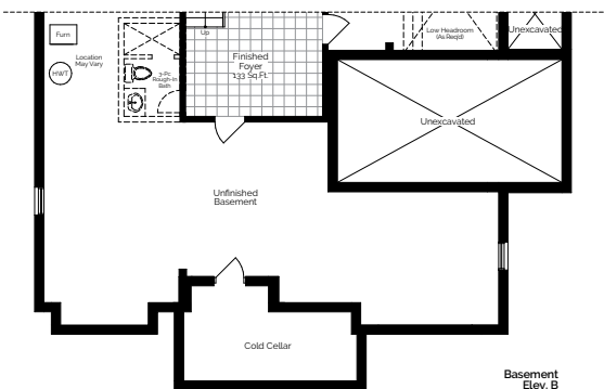
Basement Elev. B
