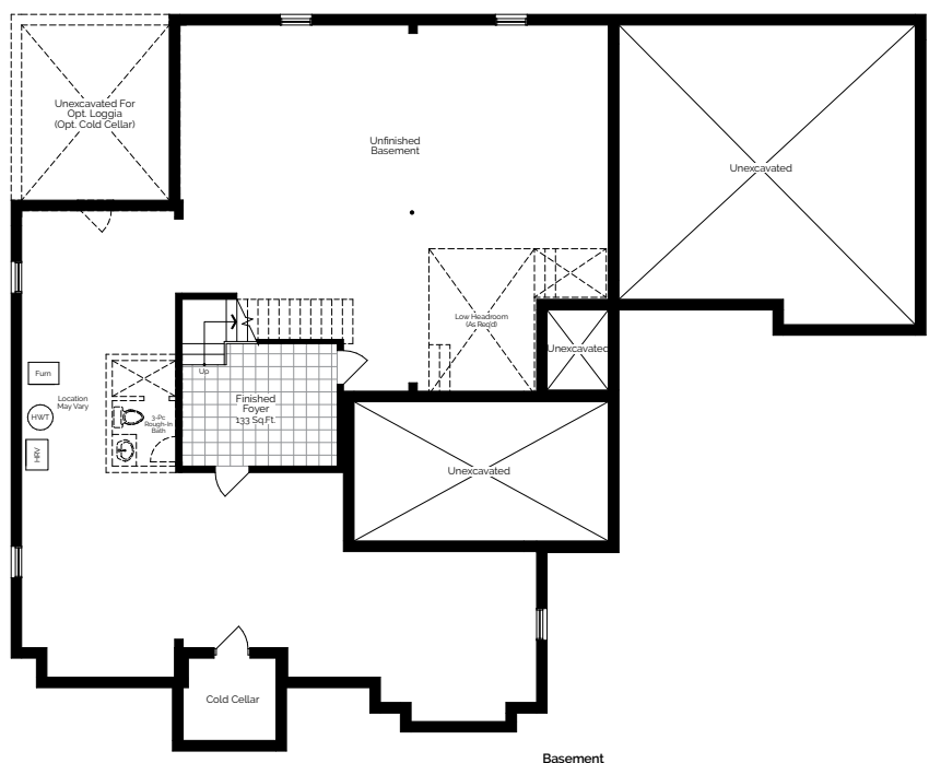
Basement Elev. A
