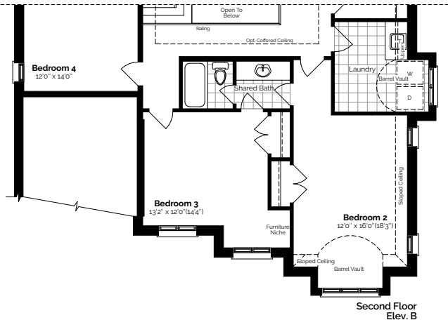
Second Floor Elev. B
