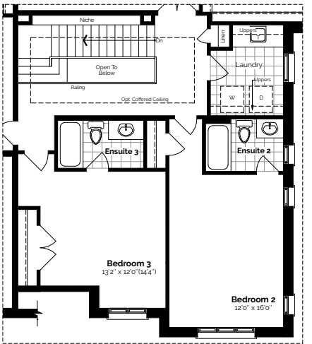
Opt. Second Floor Elev. A
