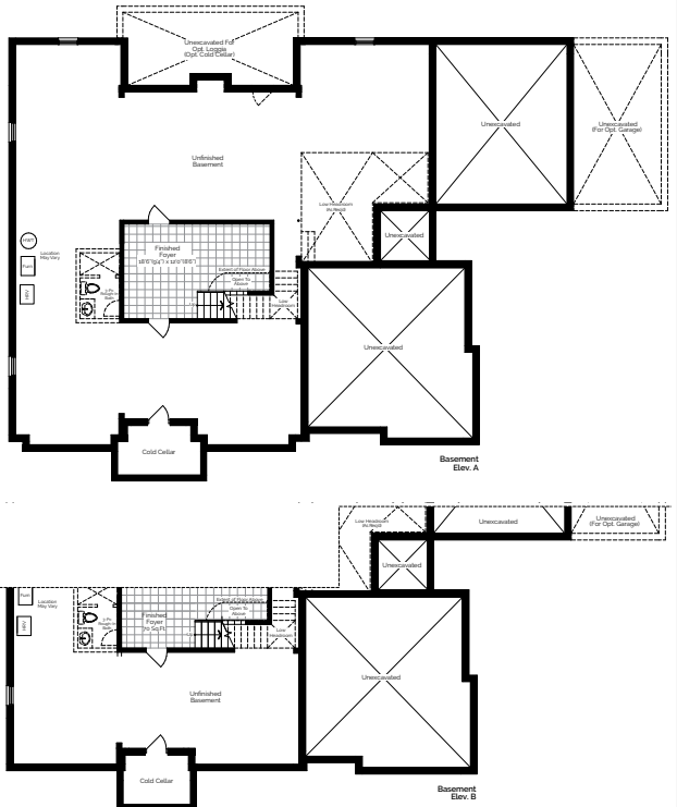
Basement Elev. A
