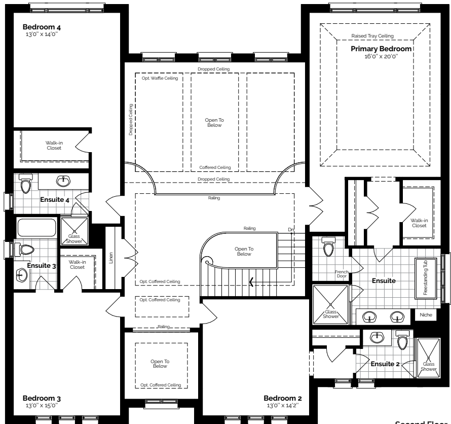
Second Floor Elev. A
